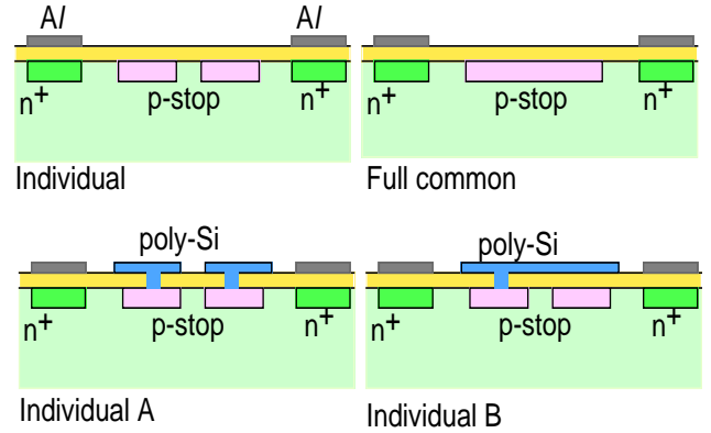
Figure 1: Four p-stop configurations of HPK n-on-n detectors.
