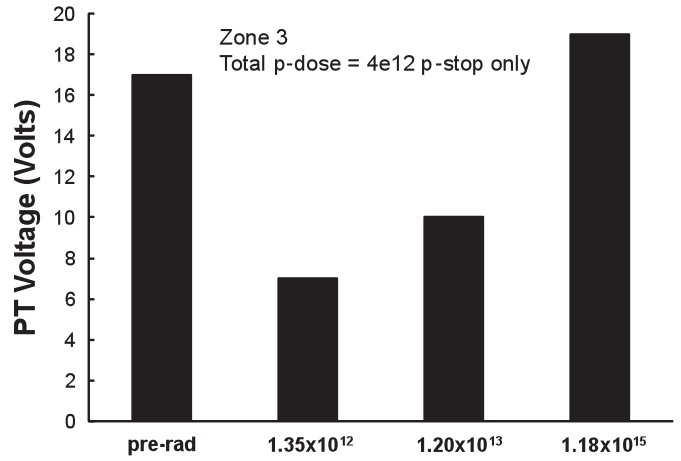
Fig. 11. Punch-through voltage for zone 3 measured at various fluences. Total p-dose = 4 \times 10^{12} cm^{-2} , fluence values are in n_{eq} .
